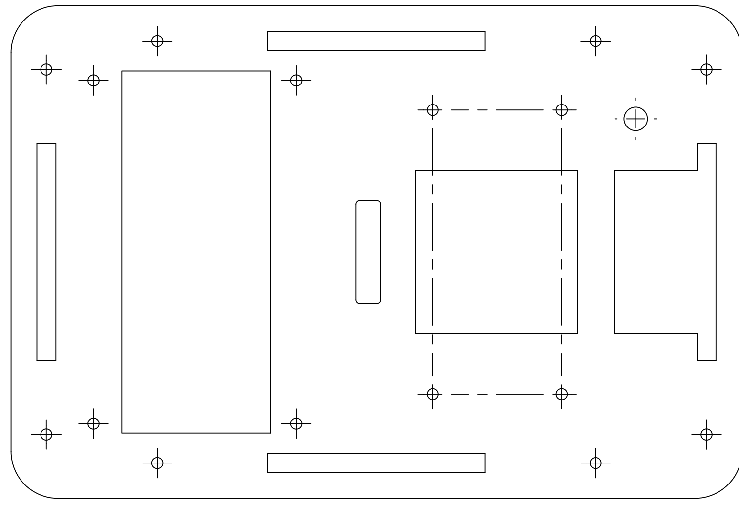
Body Top
